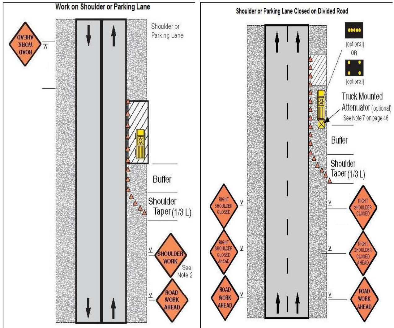
FigureA5.2andA5.3:WorkonShoulderorparkingLaneandShoulderorParking Lane Closed on Divided Road
