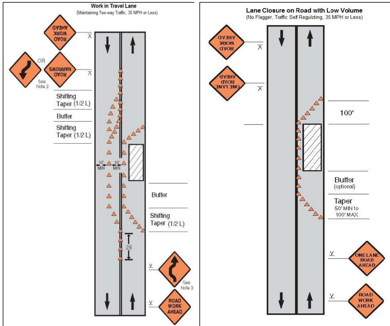
FigureA5.4andA5.5:WorkinTravelLaneandLaneClosureonRoadwithLow Volume
